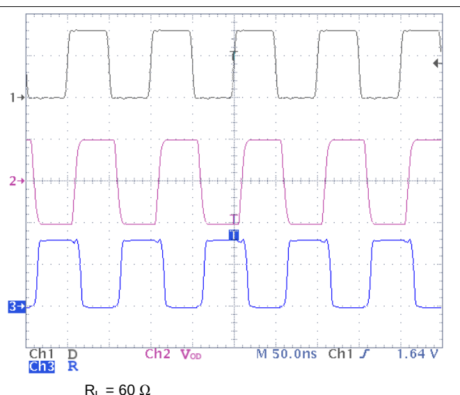
Figure 29. 65HVD75, 20 Mbps
