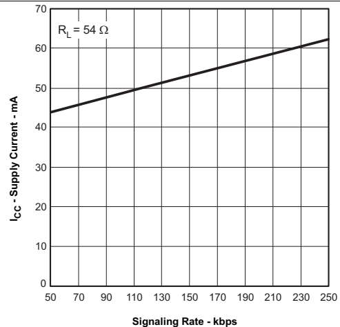
Figure 6. 65HVD72 Supply Current vs Signal Rate
